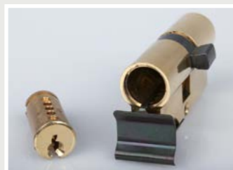
Using a dismantling clip
